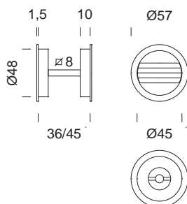
2194/S set maniglie incasso con nottolino q. 8 mm con frontale sliding door handle set with turn and release 8 mm square spindle and flush pull hole
