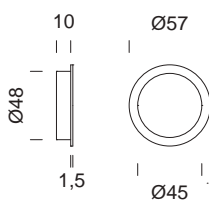
2193/S1 set maniglie incasso con frontale sliding door handle set with flush pull hole
